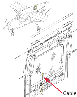
S2814-2EH Installation
